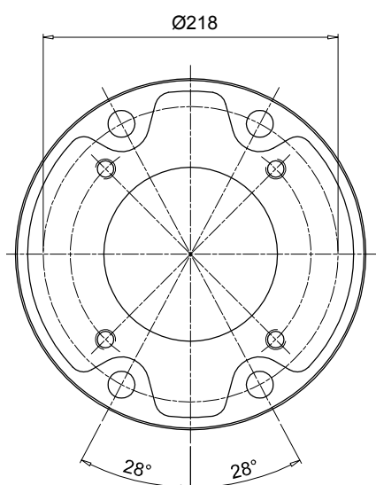
4 Bolt Version
